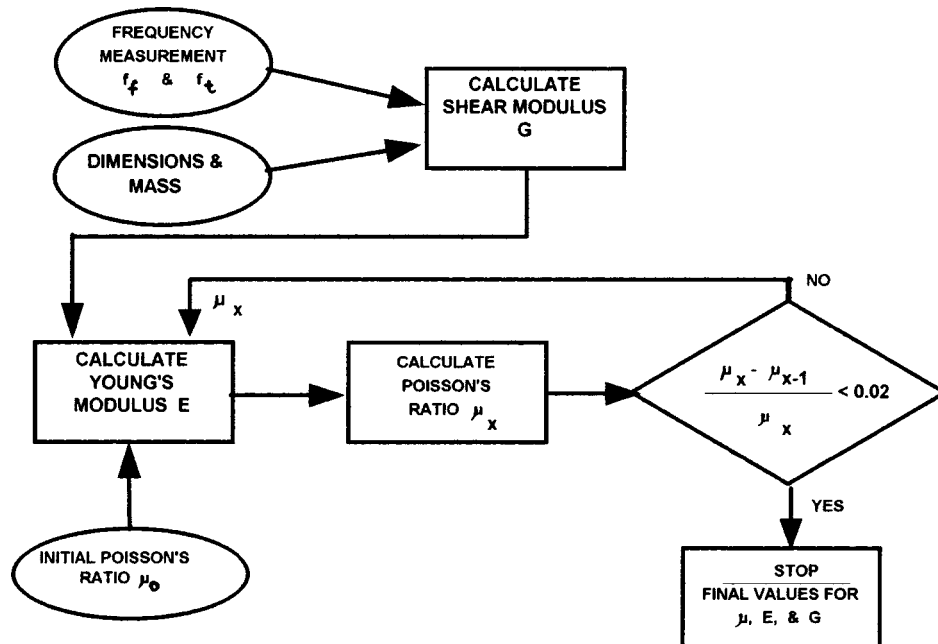
FIG. 5 Process Flow Chart for Iterative Determination of Poisson's Ratio
